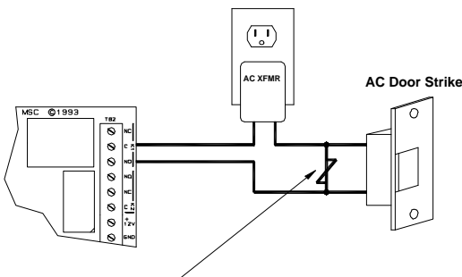
DIODE 1N4001 (50V/1A) TYPICAL
