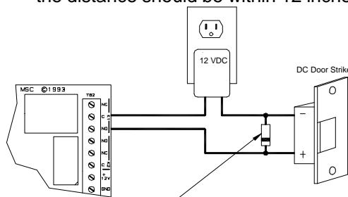
DIODE 1N4001 (50V/1A) TYPICAL
